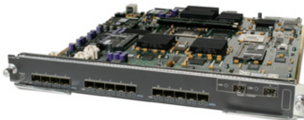
Figure 4. Cisco MDS 9000 Family Multiprotocol Storage Services Module
