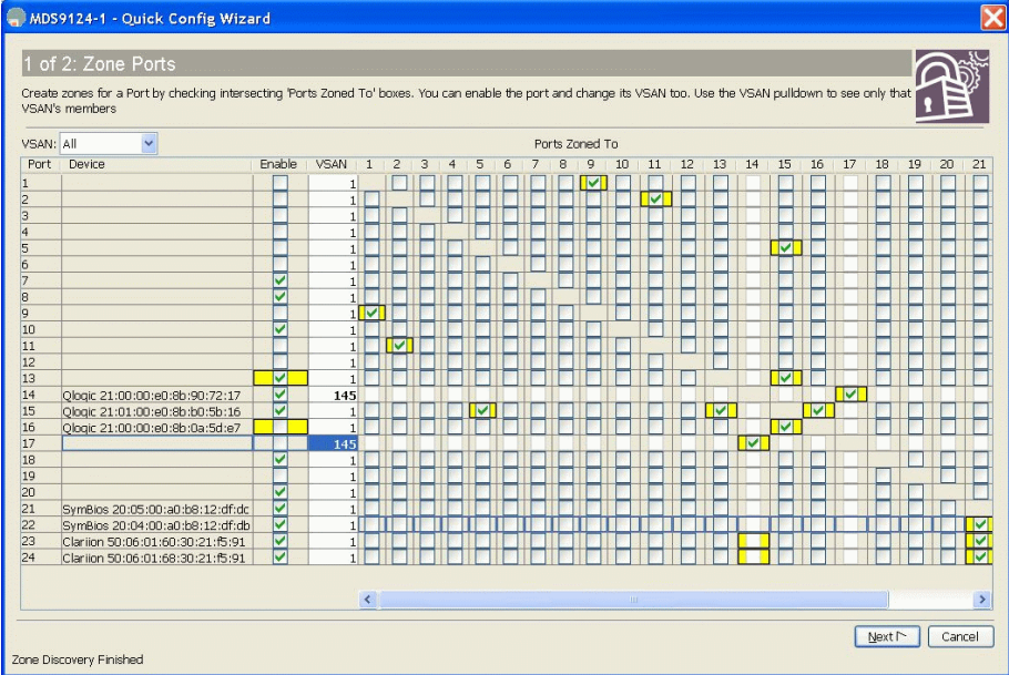
Figure 7. Quick-Configuration Wizard
