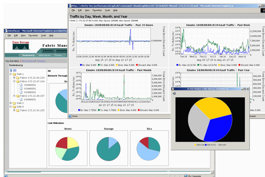
Figure 8. Performance Monitoring
